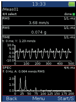
Analysator
